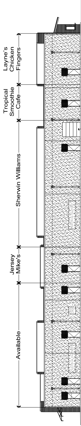
4 NORTH ELEVATION
